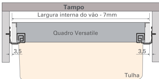
VISTA FRONTAL
