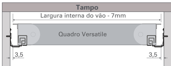
VISTA FRONTAL
